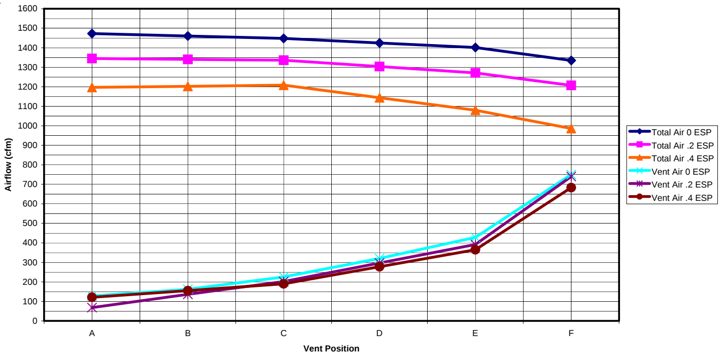
WA60 LOW SPEED TOTAL AND VENTILATION AIRFLOW
