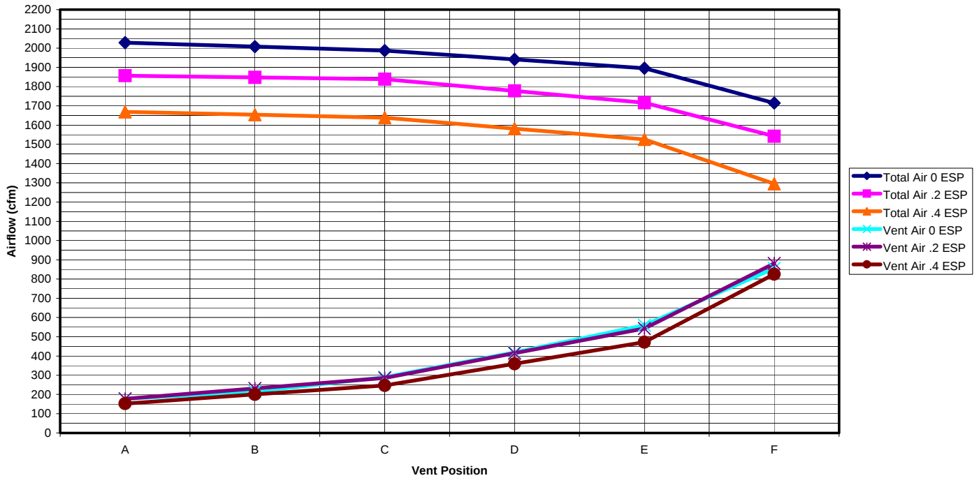
WA60 HIGH SPEED TOTAL AND VENTILATION AIRFLOW
