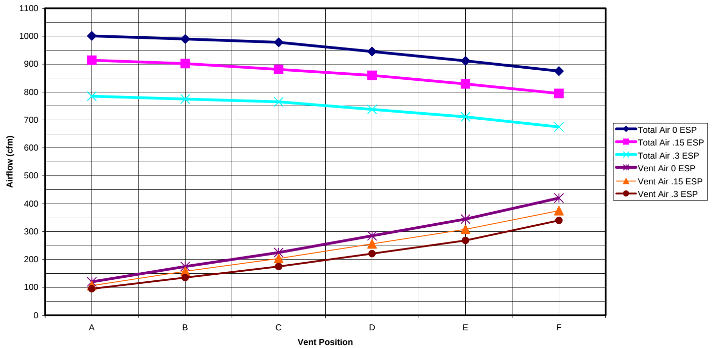
WA18, WA24 & WA25 TOTAL AND VENTILATION AIRFLOW
