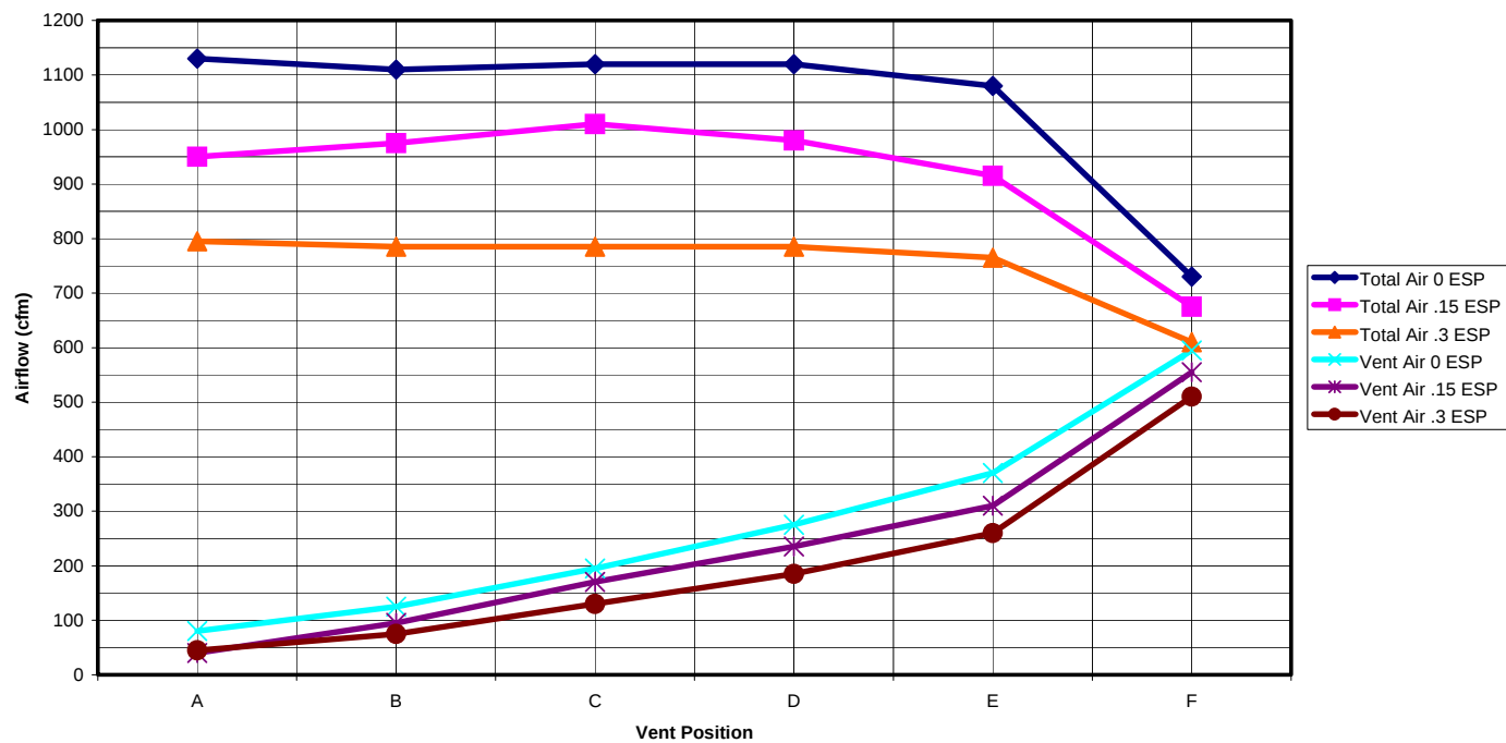
WA30 & WA37 HIGH SPEED TOTAL AND VENTILATION AIRFLOW
