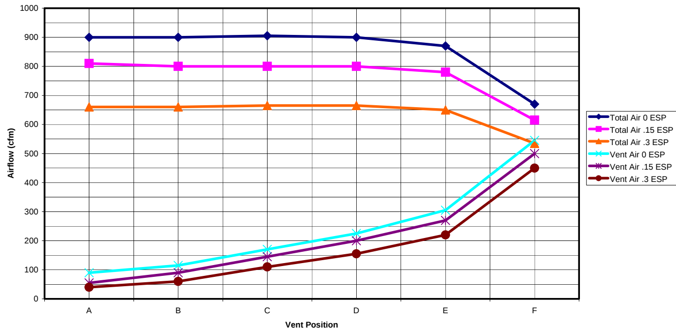
WA30 & WA37 LOW SPEED TOTAL AND VENTILATION AIRFLOW
